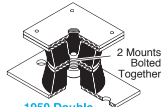
2 Mounts Bolted Together 1950 Double Deflection Design
